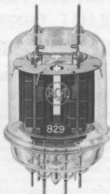
New P-P Beam Power RCA-829 takes 120 watts at the handy plate voltage of 500 volts. Goes all the way to 1½ meters. Only 4½" high and 2½" in diameter.
